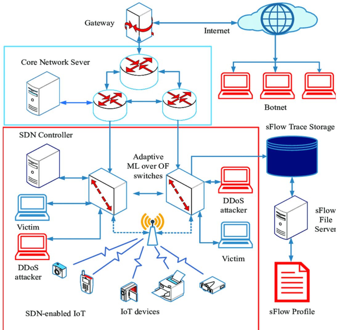
Figure 2. Architecture of deep learning in Network security management
